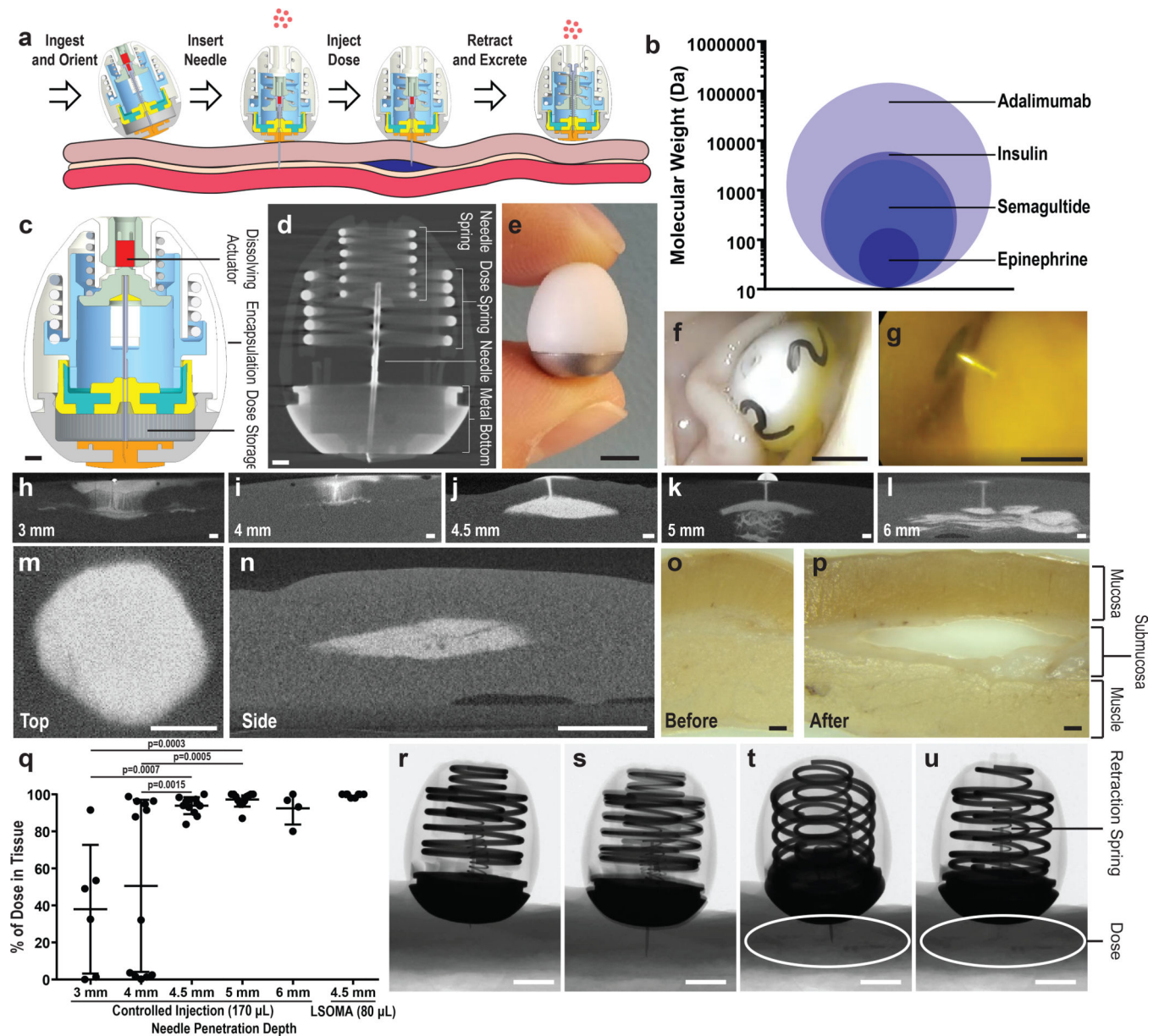
Figure 1: An oral pill for liquid drug injections into the gastric submucosa.
