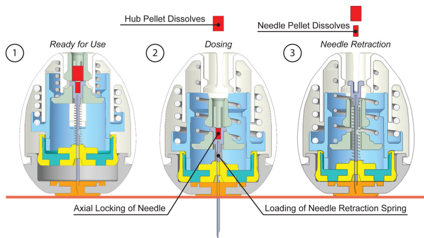
Extended Data Fig. 5: L-SOMA needle retraction mechanism design.
