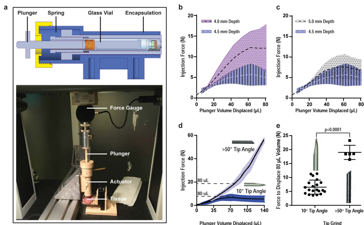
Extended Data Fig. 3: Injection test mechanism setup and ex vivo injection force calculations.
