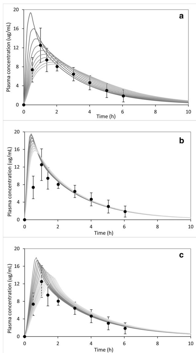
Fig. 8. Simulated plasma concentration-time profile (continuous line) in infant population representative under fasted conditions with variation of the GTT between 0.1 and 1.5 h (a), under fed conditions with different caloric intake (70–200 kcal) and adjusted GTT based on the paracetamol reference meal-dependent gastric emptying (b), and under infant fed conditions with different caloric intake (70–200 kcal) and adjusted GTT extrapolated based on the paracetamol infant formula-dependent gastric emptying (c). The color gradient represents increasing GTT values and caloric content of the meals from dark to light gray. Observed mean data and standard deviation are presented as symbols and error bars (27)
