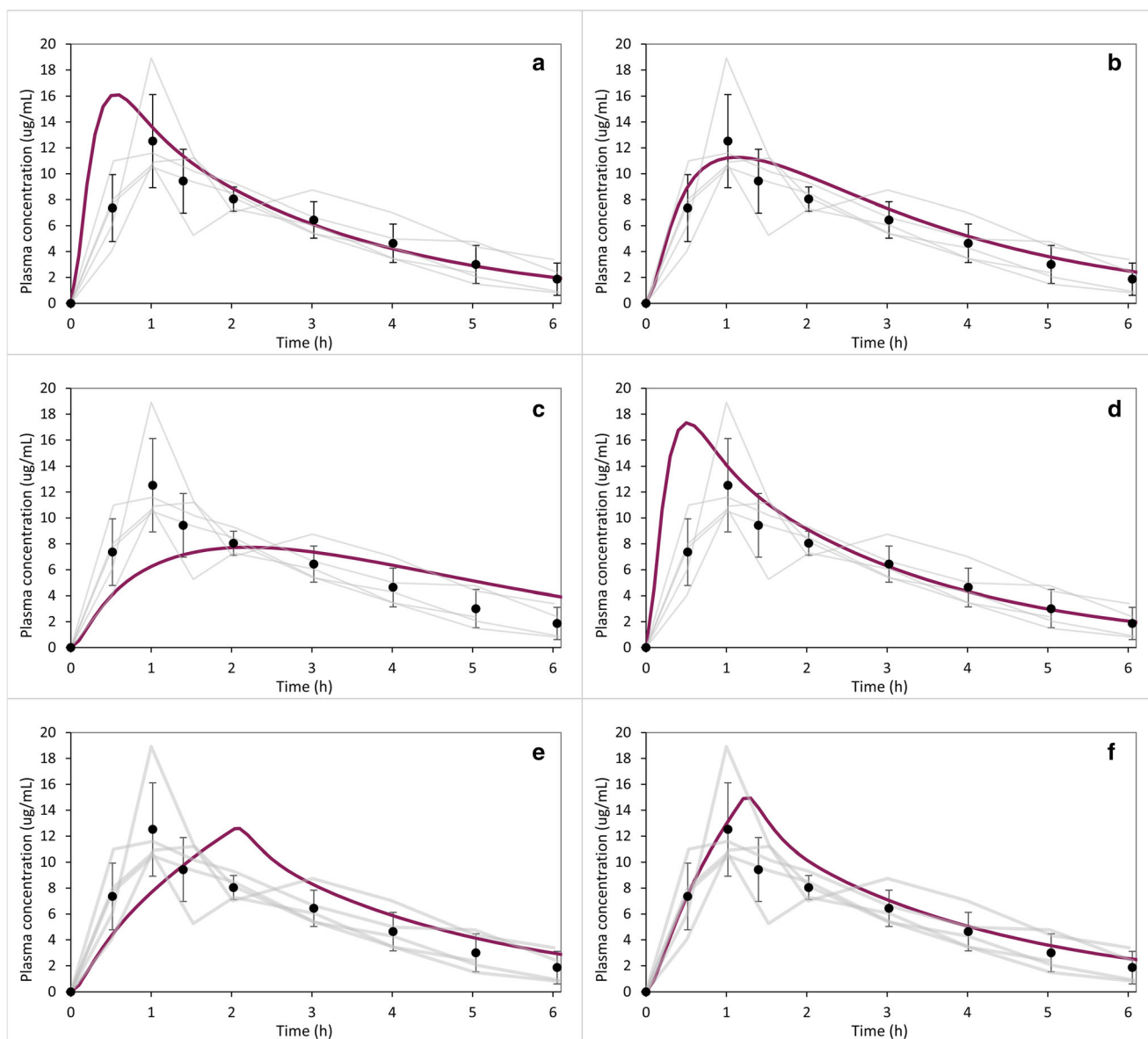
Fig. 6. Predicted plasma concentration-time profiles (purple lines) in infants under software default fasted conditions, i.e., GTT 0.1 h (a) and adjusted fasted conditions, i.e., GTT 0.75 h (b); fed conditions employing first-order GE (solid-liquid meal) and software default GTT value of 2.1 h (c) or adjusted GTT value of 0.21 h (d); infant formula-fed conditions following zero-order GE kinetics (liquid homogeneous meals) using software default GTT value of 2.1 h (e) or adjusted GTT value of 1.21 (f). Observed mean concentrations and standard deviations depicted as symbols and error bars; individual observed data is presented with gray lines (27)
