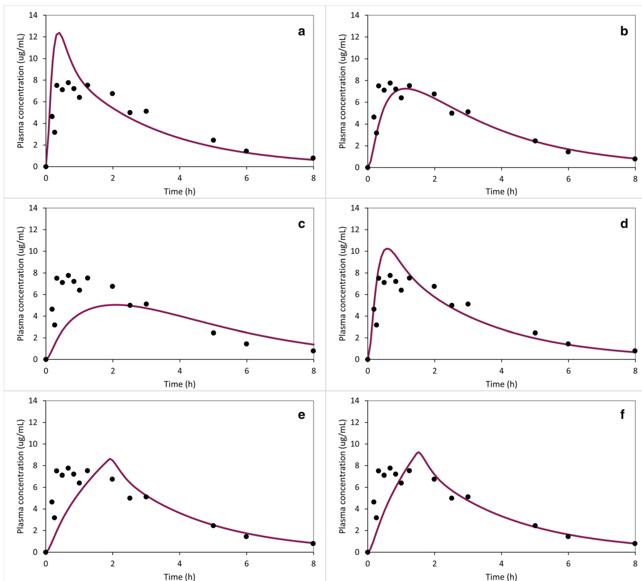
Fig. 7. Predicted plasma concentration-time profiles (purple lines) in infants under software default fasted conditions, i.e., GTT 0.1 h (a) and adjusted fasted conditions, i.e., GTT 0.75 h (b); fed conditions employing first-order GE (solid-liquid meal) employing software default GTT value of 1.89 h (c) and adjusted GTT value of 0.26 h (d); infant formula-fed conditions following zero-order GE kinetics (liquid homogeneous meals) using software default GTT value of 1.89 h (e) and adjusted GTT value of 1.47 (f). Observed mean concentrations depicted as symbols (28)
