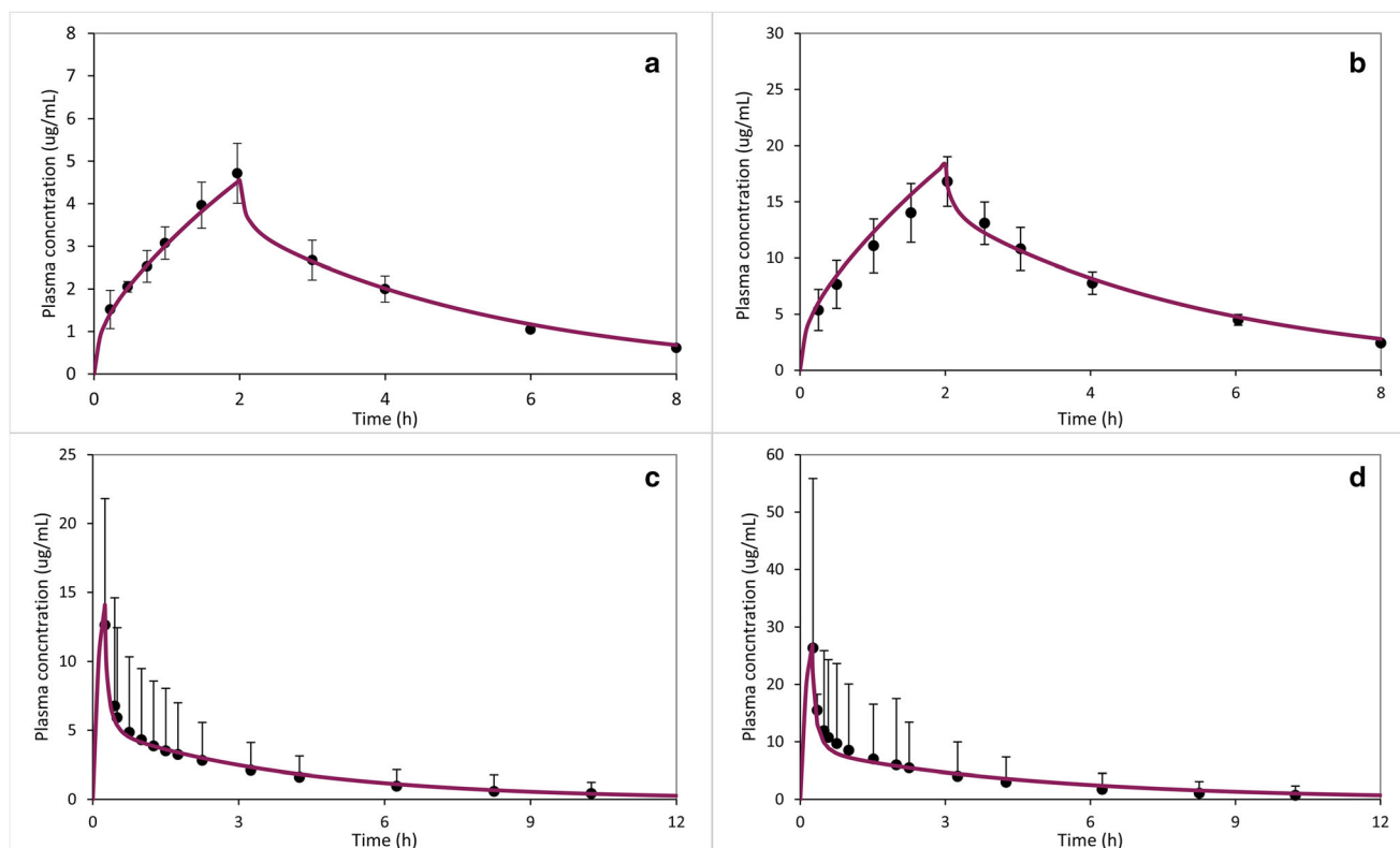
Fig. 2. Simulations of paracetamol plasma concentrations following i.v. administration in healthy adults. The disposition model was developed according to data observed at a low (a) (5 mg/kg, i.e., 350 mg) and high dose (b) (20 mg/kg, i.e., 1400 mg) (16). Model verification was performed with clinical datasets not used during model development at low 500 mg (c) and high 1000 mg (d) doses (15). Symbols denote observed mean data, error bars represent the standard deviation of the observed data, and continuous lines represent the simulated plasma concentration-time profile
