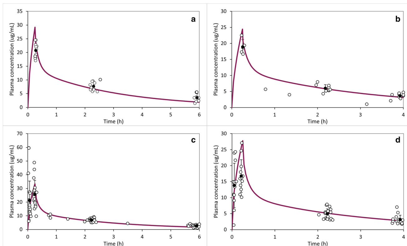
Fig. 5. Simulated plasma concentration-time profiles (continuous purple lines) in infants ( a, b ) and in children ( c, d ) after i.v. administration of paracetamol at doses 15 mg/kg ( a, c ) or 12.5 mg/kg ( b, d ). Observed mean concentrations and standard deviations depicted as black symbols and error bars; individual concentrations ( n = 25 infants and n = 56 children and adolescents) are depicted with open symbols (25)
