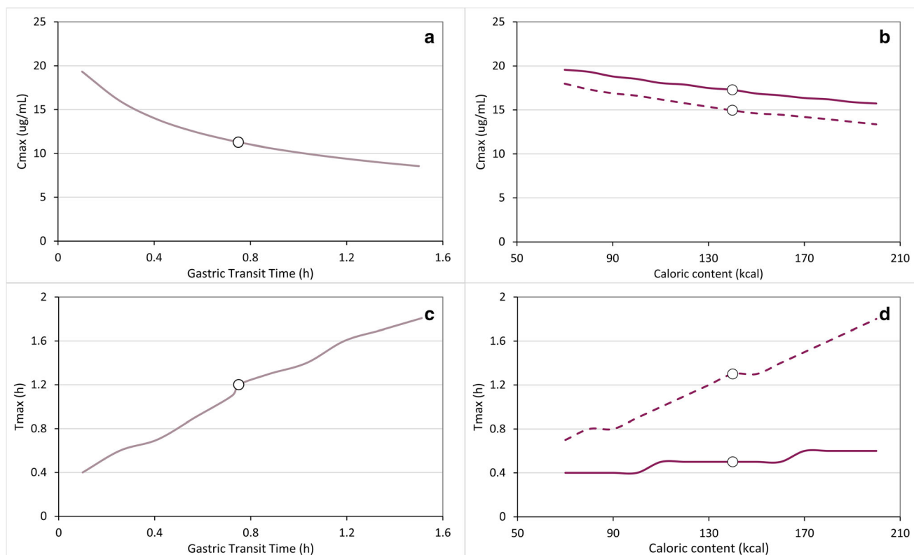
Fig. 9. Parameter sensitivity analysis for Cmax and Tmax results in a population representative infant (4 months old (27)) as a function of GTT under adjusted fasted conditions (a, c), or caloric content (GTT) influence under adjusted reference meal conditions (continuous lines b and d), or caloric content influence under adjusted infant formula-fed conditions (discontinuous lines b and d). Values used within the pediatric simulations employing adjusted MGTT values are shown as open circles
