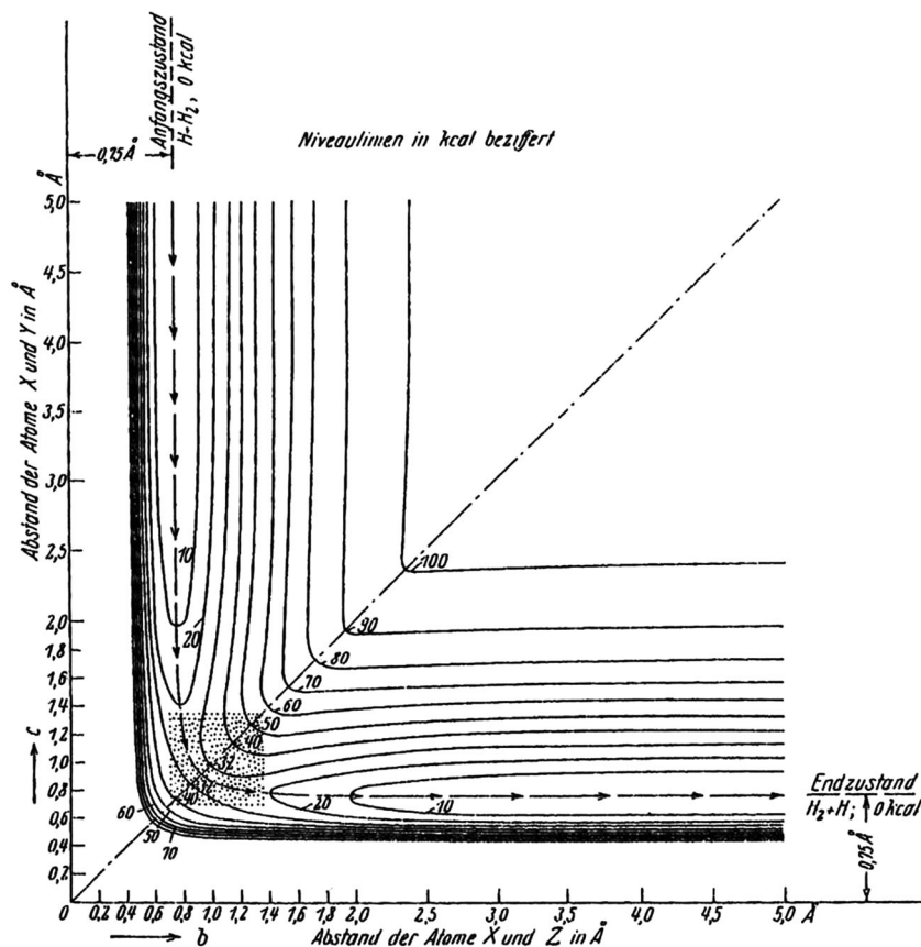
Figure 15. Hypersurface potential for the reaction H + H_2 \rightarrow H_2 + H as a function of both distances b and c according to Eyring and Polanyi. [22]
