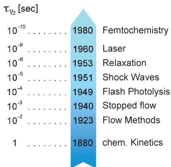
Figure 14. Chronology for the development of experimental methods to determine the half-lives \tau_{1/2} of chemical reactions.
