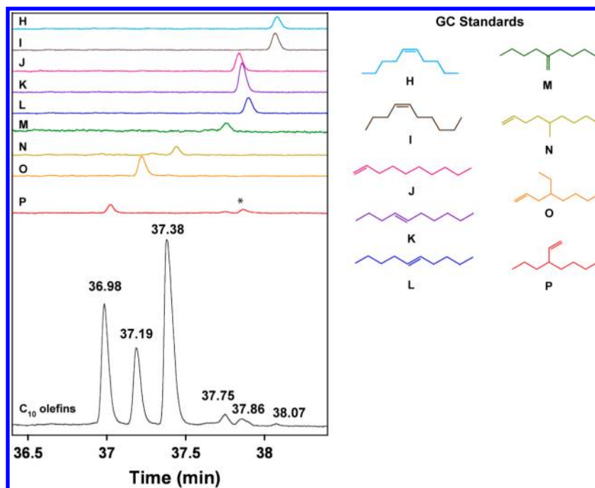
Figure 1. Gas chromatogram of the C 10 alkenes (black, bottom trace) obtained by fractional distillation from the reaction of 1/MMAO/ethylene/1-hexene. The products appear at 36.98, 37.19, 37.38, 37.75, 37.86, and 38.07 min. The C 10 olefin standards are shown directly above (from top to bottom, RT = retention time in min): cis -5-decene (H, light blue; 38.08); cis -4-decene (I, brown; 38.07); 1-decene (J, pink; 37.84); trans -4-decene (K, purple; 37.86); trans -5-decene (L, blue; 37.90); 2-butyl-1-hexene (M, green; 37.76); 5-methyl-1-nonene (N, yellow; 37.44); 4-ethyl-1-octene (O, orange; 37.22); 3-propyl-1-heptene (P, red; 37.02). The peak marked with an asterisk (*) is the trans -4-decene impurity present in the 3-propyl-1-heptene standard (see the Supporting Information).
