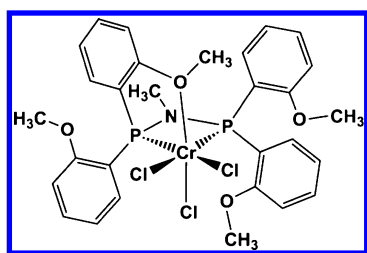
Chart 1. Structure of the Chromium Precatalyst [\text{CrCl}_3(\text{PNP}^{\text{OMe}})] ( 1 )
