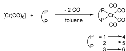
Scheme 3 Synthetic route to complexes 4–6 .
