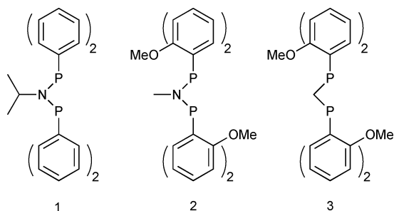
Fig. 1 Ligand derivatives.
