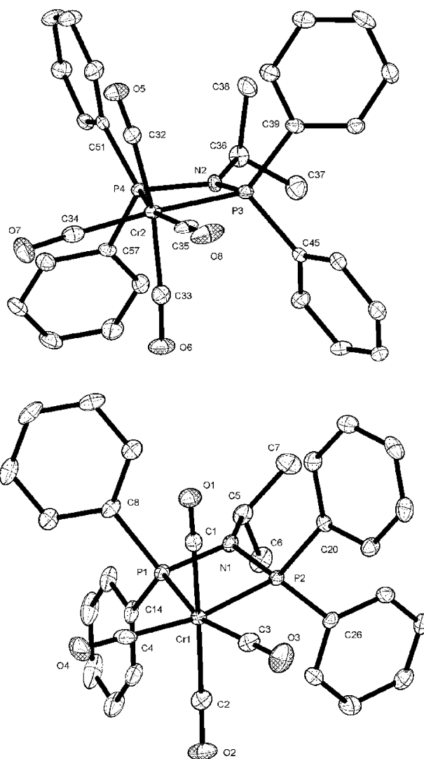
Fig. 2 Molecular structure and numbering scheme for [\text{Cr}(\text{CO})_4(\text{Ph}_2\text{PN}(\text{iPr})\text{PPh}_2)] 4 (Hydrogen atoms omitted for clarity; ORTEP plots created at 50% probability).
