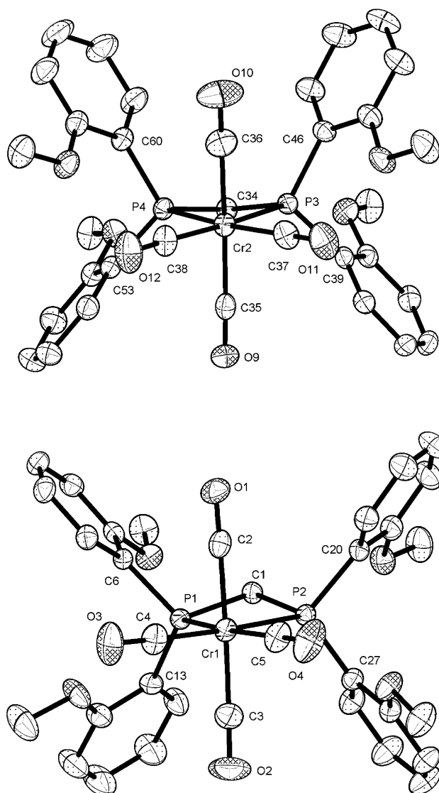
Fig. 4 Molecular structure and numbering scheme for [\text{Cr}(\text{CO})_4\text{-(Ar}_2\text{PCH}_2\text{PAR}_2)] 6 (Hydrogen atoms omitted for clarity; ORTEP plots created at 50% probability).
