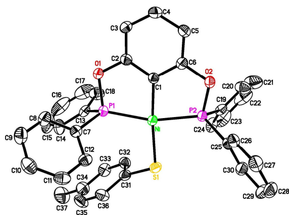
Fig. 1 ORTEP drawing of [2,6-(\text{Ph}_2\text{PO})_2\text{C}_6\text{H}_3]\text{NiSC}_6\text{H}_4\text{CH}_3 ( 1b ) at the 50% probability level. Hydrogen atoms are omitted for clarity. Selected bond length (Å) and angles (deg): Ni–S1 = 2.1947(7), Ni–C1 = 1.907(2), Ni–P1 = 2.1555(7), Ni–P2 = 2.1452(7), S1–C31 = 1.784(3); P1–Ni–P2 = 163.10(3), P1–Ni–S1 = 103.11(3), P2–Ni–S1 = 93.79(3), C1–Ni–S1 = 174.45(7), C31–S1–Ni = 110.85(8).
