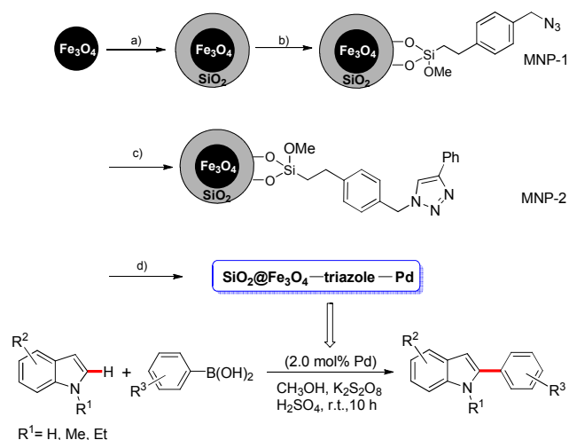
Scheme 1 Preparation of magnetic nanoparticles-supported palladium catalyst and its application in C-2 arylation of indoles.
