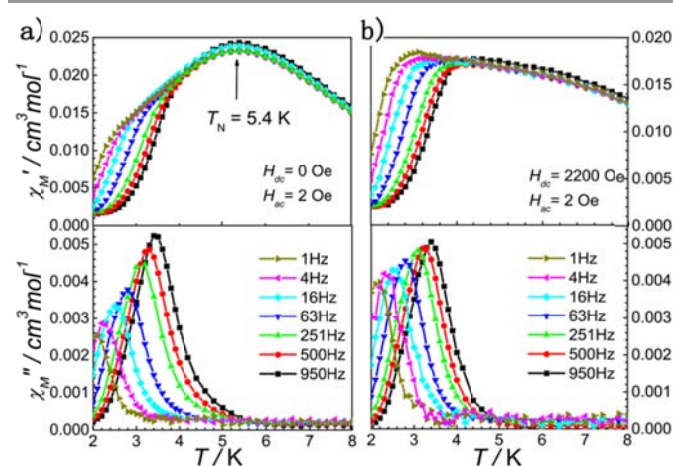
Fig. 4 The real ( \chi' ) and imaginary ( \chi'' ) parts of the ac susceptibilities for 1 in zero (a) and 2200 Oe dc field (b).
