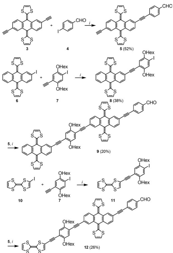
Scheme 1 Reagents and conditions used in the synthesis of 1 and 2 : (i) Pd(PPh 3 ) 4 /CuI/iPr 2 NH/THF/Δ.
