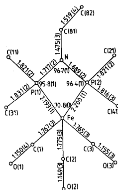
Fig. 1. Atomic numbering and selected bond lengths (Å) and angles ( ^\circ ). The phenyl rings attached to the pivot atoms C(11), C(21), C(31) and C(41) are not shown.
