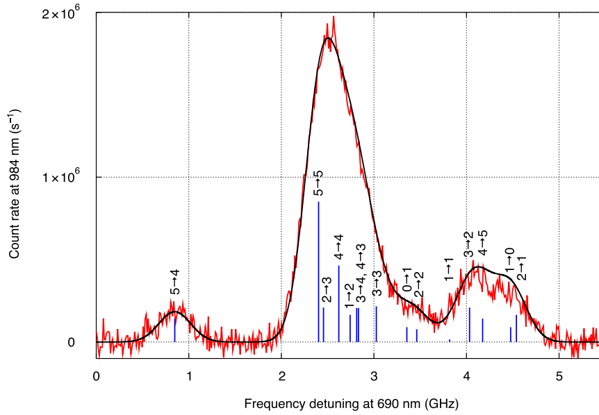
Extended Data Fig. 1 | Doppler-broadened spectrum of the 5f^2 F_{5/2} \leftrightarrow 6d^2 D_{5/2} transition of ^{229}\text{Th}^{3+} . The red curve represents the background-subtracted fluorescence count rate at 984 nm as a function of the 690-nm laser frequency. Vertical blue bars denote hyperfine transitions ( F_g^i \rightarrow F_g^f ) whose frequencies were calculated on the basis of refs. 7,8. The relative height of the blue bars
