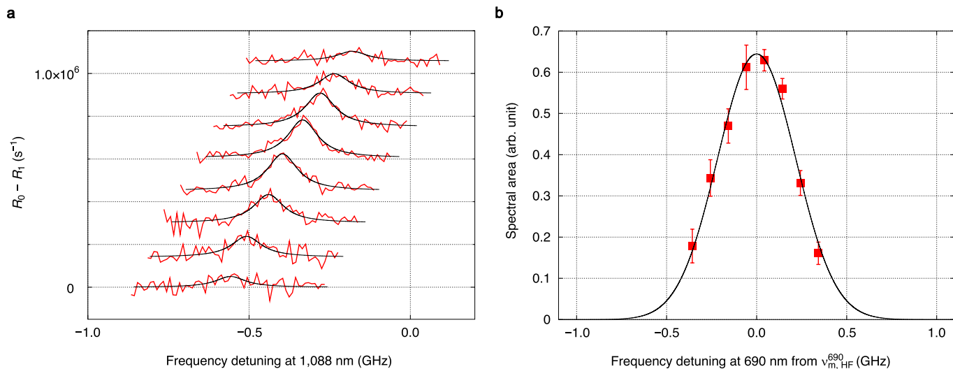
Extended Data Fig. 3 | Determination of the resonance frequency ( \nu_{m, HF}^{690} ) of the |5f^2F_{5/2}, F_m=1\rangle \rightarrow |6d^2D_{3/2}, F_m=2\rangle transition. a , The spectra of the |5f^2F_{5/2}, F_m=1\rangle \rightarrow |6d^2D_{3/2}, F_m=2\rangle transition (1,088 nm) were measured with several 690-nm laser frequencies around the resonance frequency of the |5f^2F_{5/2}, F_m=1\rangle \rightarrow |6d^2D_{3/2}, F_m=2\rangle transition. From bottom to top, the 690-nm laser frequency was increased by 100 MHz at each step. The spectra were
