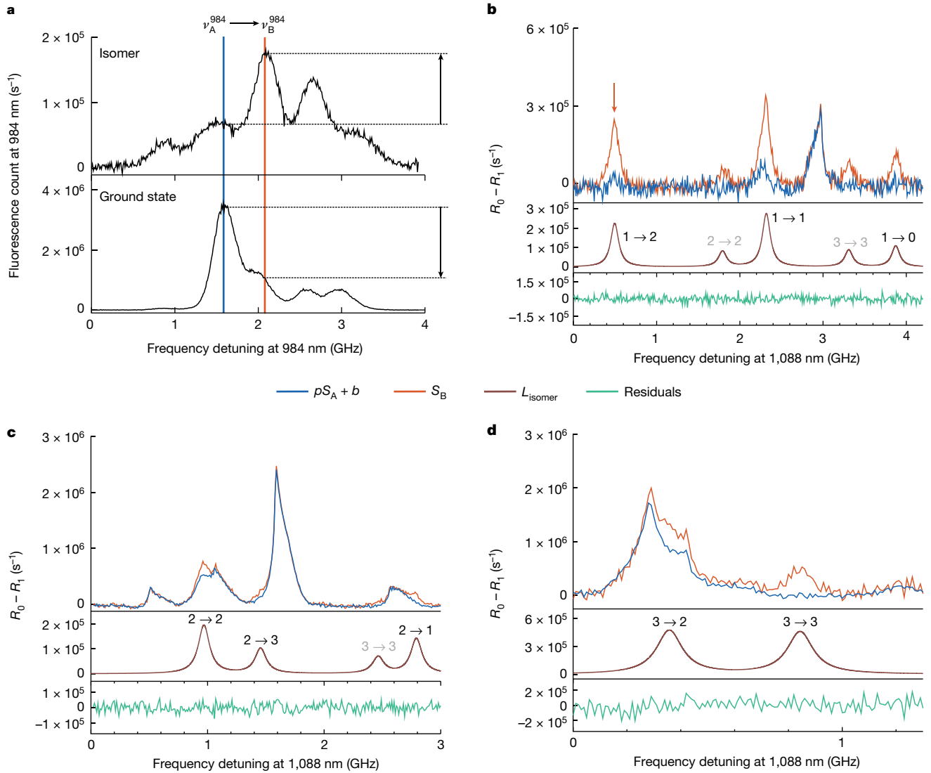
Fig. 3 | Observation of the hyperfine spectra of ^{229\text{m}}\text{Th}^{3+} . a , Spectra of the 984-nm fluorescence transition are separately shown for ^{229}\text{Th}^{3+} in the nuclear ground state and isomer. The difference in fluorescence strength between the two nuclear states at \nu_A^{984} and \nu_B^{984} allowed detection of the isomer signal. b–d , We determined the hyperfine constants A_m and B_m of the 6d^2D_{3/2} state of ^{229\text{m}}\text{Th}^{3+} by fitting pS_A + b + L_{\text{isomer}} to S_B . Here S_A and S_B are the hole-burning spectra of the 1,088-nm transition taken with \nu_A^{984} and \nu_B^{984} , respectively. The 690-nm laser was tuned to the (b) |5f^2F_{5/2}, F_m = 1\rangle \rightarrow |6d^2D_{3/2}, F_m = 2\rangle (b), 2 \rightarrow 3 (c) and 3 \rightarrow 3 (d) transitions. L_{\text{isomer}} represents a group of Lorentzian curves describing the isomer peaks. The hyperfine constants were determined
