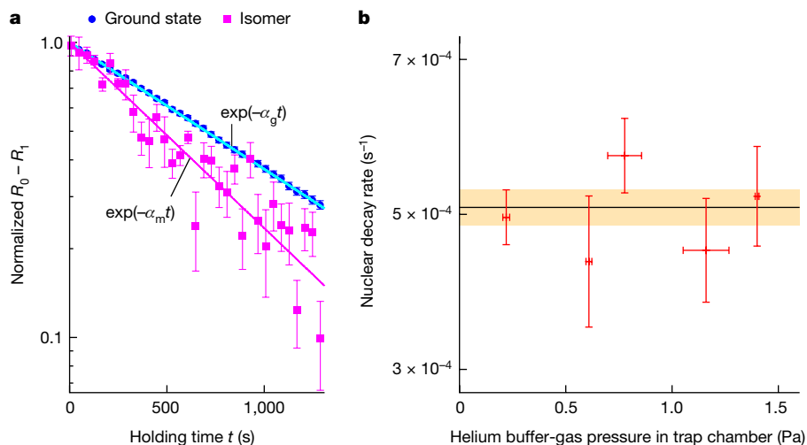
Fig. 4 | Determination of the nuclear decay rate of ^{229\text{m}}\text{Th}^{3+} . The nuclear decay rate of ^{229\text{m}}\text{Th}^{3+} was determined by taking the difference in the decay rates between ^{229\text{g}}\text{Th}^{3+} (ground state) and ^{229\text{m}}\text{Th}^{3+} (isomer). a , Decay data are shown as functions of the ion holding time t . Both decay data were fitted by a single exponential function ( \exp(-\alpha t) ) to determine the decay rate \alpha (cyan and
