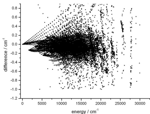
Fig. 2. Differences between the present MARVEL energy levels and their counterparts present in the BT2 list [194].
