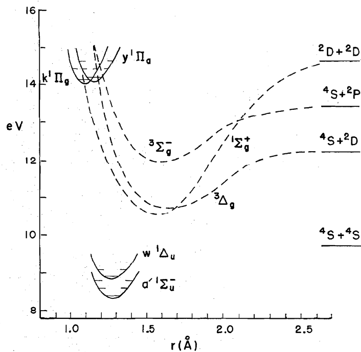
FIGURE 3. Potential curves for states involved in transitions to and interactions with the k^1\Pi_g and y^1\Pi_g states. These are discussed section 8.9.
