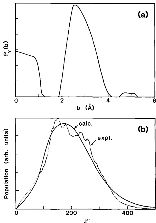
FIG. 12. (a) The specific opacity function for the Ba + HI \rightarrow BaI( \nu = 8 ) + H system, assuming that there exists an activation energy of 0.5 kcal/mol. (b) The experimental (dot) and calculated (solid line) rotational distributions for the reaction studied using the specific opacity function shown in (a).
