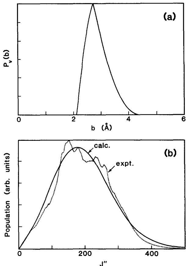
FIG. 8.(a) The specific opacity function for the Ba + HI \rightarrow BaI( \nu=8 ) + H system, assuming there is no velocity dependence for the reaction. (b) The experimental (dot) and calculated (solid line) rotational distributions for the reaction studied using the specific opacity function shown in (a).
