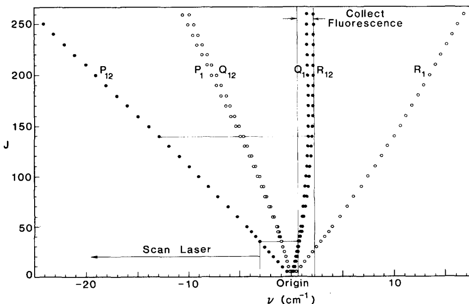
FIG. 3. A Fortrat diagram of the BaI C^2\Pi_{1/2}-X^2\Sigma^+ system. Closed dots represent transitions involving f level upper states ( \Lambda -doubling components), and open dots represent transitions involving e level upper states. When a monochromator collects fluorescence only in the Q_1 + R_{12} bandhead region, the excitation of the P_{12} transitions can be selectively detected.
