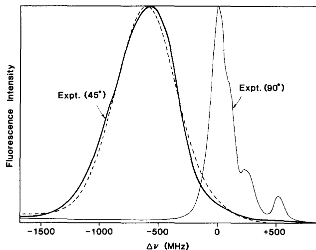
FIG. 6. A Doppler-shift spectrum of the Ba 1P^*-1S_0 transition. The broken line is the calculated line profile using the Ba velocity distribution given by Eq. (10).
