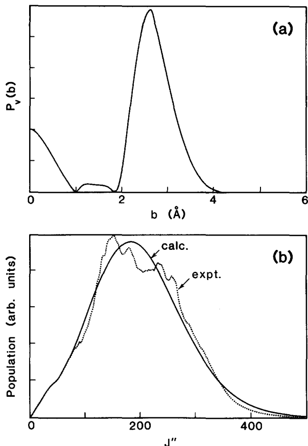
FIG. 10. (a) The specific opacity function for the Ba + HI \rightarrow BaI( \nu = 8 ) + H system, assuming that the reaction probability varies as v_{rel}^{1/2} . (b) The experimental (dot) and calculated (solid line) rotational distributions for the reaction studied using the specific opacity function shown in (a).
