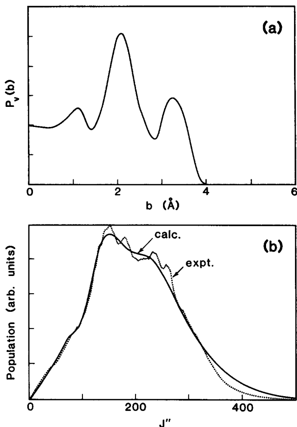
FIG. 13. (a) The specific opacity function for the Ba + HI \rightarrow BaI( \nu = 8 ) + H system, assuming that there exists an activation energy of 2.0 kcal/mol. (b) The experimental (dot) and calculated (solid line) rotational distributions for the reaction studied using the specific opacity function shown in (a).
