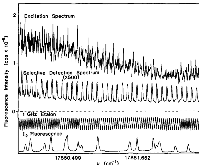
FIG. 2. A 3 \text{ cm}^{-1} segment of the BaI C^2\Pi_{1/2}-X^2\Sigma^+(8,8) excitation spectrum (upper trace) and the selectively detected laser-induced fluorescence spectrum (middle trace). An I_2 fluorescence spectrum and 1 GHz etalon markers, which were used to calibrate wavelengths, are shown in the lower two traces.
