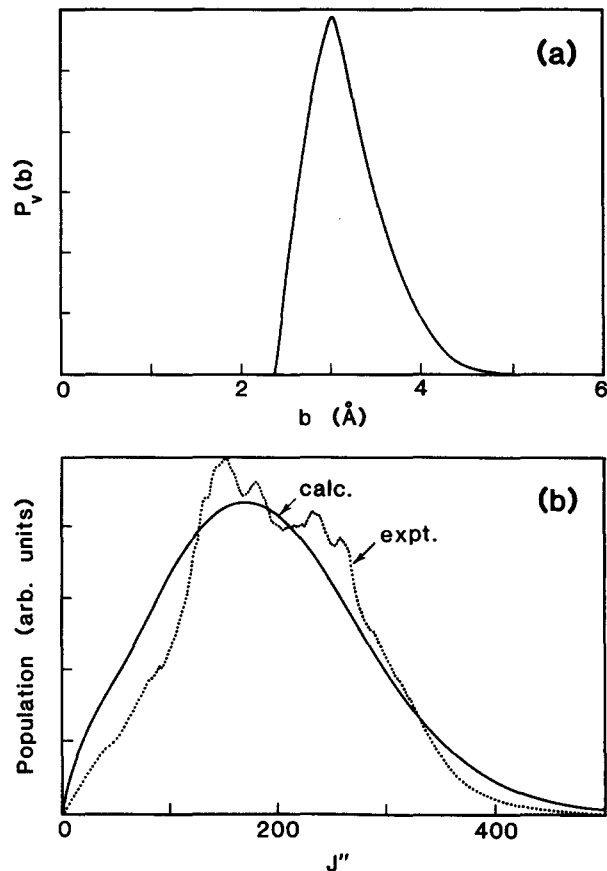
FIG. 9.(a) The specific opacity function for the Ba + HI \rightarrow BaI( \nu=8 ) + H system, assuming that the reaction probability varies as v_{\text{rel}}^{-1/2} . (b) The experimental (dot) and calculated (solid line) rotational distributions for the reaction studied using the specific opacity function shown in (a).
