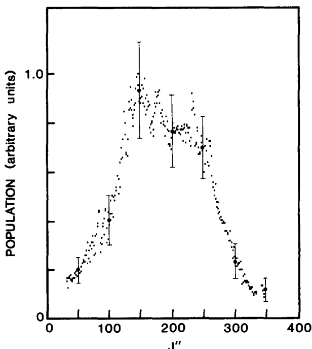
FIG. 7. The rotational distribution (unsmoothed) of the BaI product in \nu = 8 produced by the Ba + HI beam-gas reaction.
