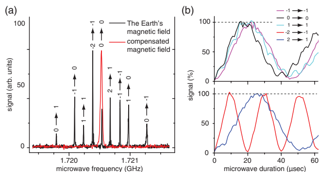
FIG. 2. (a) Frequency scan over the |X, f, +, F=2\rangle \rightarrow |X, e, -, F=1\rangle transition in the presence of the earth's magnetic field (black) and the compensated magnetic field (red). Spectra are scaled to each other to facilitate a better comparison. The nine |X, f, +, F=2, M_F\rangle \rightarrow |X, e, -, F=1, M_F\rangle transitions are indicated. (b) Rabi oscillations of selected |X, f, +, F=2, M_F\rangle \rightarrow |X, e, -, F=1, M_F\rangle transitions.
