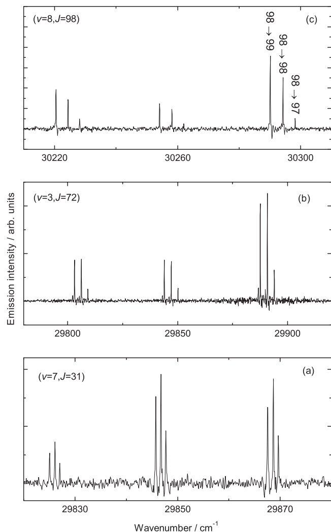
FIG. 8. Part of the FT E0_g^+(^3P_2) \rightarrow A1_u emission following excitation of (a), E(v=7, J=31) , (b), E(v=3, J=72) , and (c), E(v=8, J=98) .
