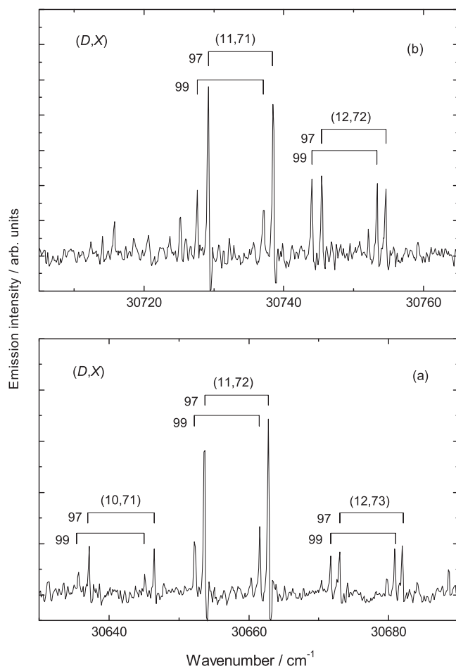
FIG. 4. Two segments of the FT DO_u^+(^3P_2) \rightarrow X0_g^+ emission following the excitation of E(v=8, J=98) . The labels identify vibrational quantum numbers in the (D,X) bands and rotational numbering in the DO_u^+(^3P_2) state.
