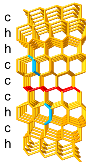
FIG. 3. Hydrogen-bonded network of stacking disordered ice I (ice Isd). Hexagonal and cubic stacking are indicated by “h” and “c,” respectively. One of the layers is shown in red. The different conformations of the six-membered rings resulting from the two types of stacking are highlighted in cyan.
