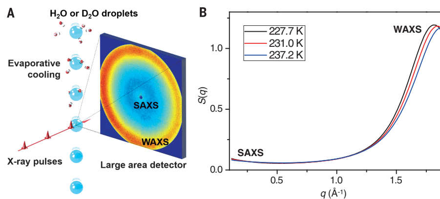
Fig. 1. Single-shot x-ray scattering of supercooled H_2O and D_2O under evaporative cooling conditions at the PAL-XFEL facility. (A) Schematic diagram of the experimental setup. A continuous series of droplets, each with a uniform diameter of \sim 14 \mu m , was generated by a droplet dispenser in vacuum, and the scattering patterns were generated by x-ray pulses with a photon energy of 5.5 keV. Various temperature points were measured by changing the distance between the dispenser and the measurement point. (B) Temperature-dependent scattering structure factor of H_2O . The wide dynamic range of the detector (MX225-HS, Rayonix) allows us to simultaneously measure the SAXS and WAXS regions for each x-ray shot. Data from three different temperature points (227.7, 231.0, and 237.2 K) are shown as examples.
