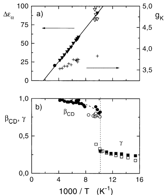
Figure 6. The parameters of the Cole–Davidson function as a function of 1000/T . (a) Left-hand axis: the relaxation strength \Delta\varepsilon_\alpha for the supercooled liquid (full triangles) and the plastic crystal (open triangles). The data point at room temperature (filled circle) has been derived from an evaluation of the data in [22]. The straight line represents the behaviour \Delta\varepsilon_\alpha(T) = a + b/T . Right-hand axis: the temperature dependence of the Kirkwood correlation factor g_K (+) as given by equation (5). (b) The width parameter \beta_{CD} (circles) and the exponent \gamma (squares) of the high-frequency power law of the main relaxation for the plastic crystal (open symbols) and the supercooled liquid (full symbols). The dotted line indicates T_g .
