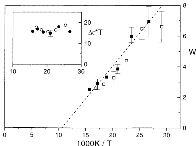
Figure 8. The temperature dependence of the parameters (relaxation strength \Delta\epsilon : circles; width w : squares) describing the secondary relaxation (open symbols: glassy crystal; filled symbols: structural glass). The dashed line is a fit to equation (8).
