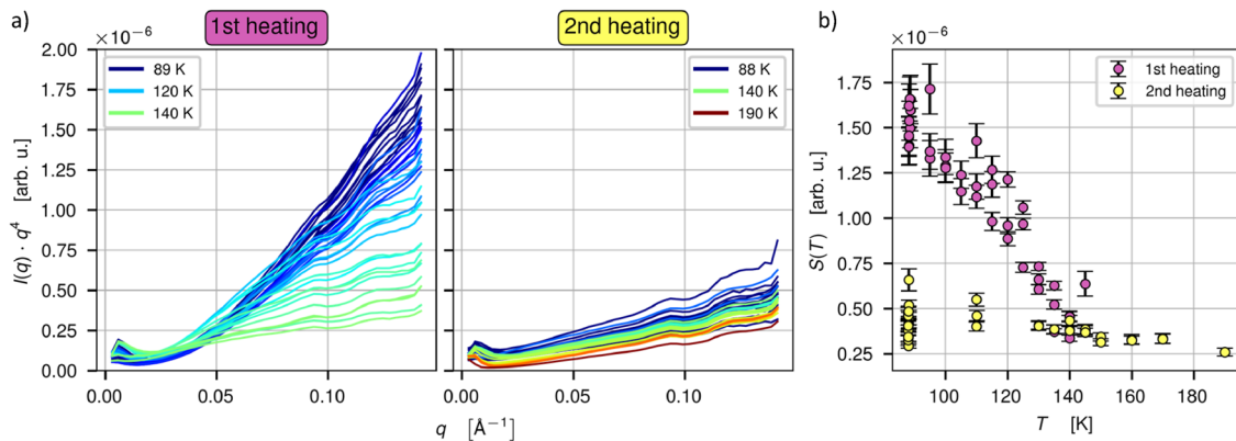
FIG. 2. X-ray scattering intensity showing the change in morphology during heating. (a) The scattering intensity is scaled by q^4 to show the specific surface area as the asymptotic tendency according to Porod's law. The temperature is increased in increments of 5 K during the first heating. During the second heating, the temperatures are 88, 110, and 130 K, followed by 5 K increments up to 190 K. (b) Specific surface area S calculated as the average of I \cdot q^4 over the range 0.12\text{--}0.14 \text{ \AA}^{-1} . This dataset was collected in SAXS geometry.
