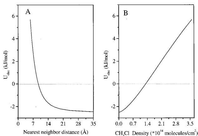
FIG. 5. (A) The calculated values of U_{\text{elec}} vs nearest neighbor separation distance. (B) Values calculated vs \text{CH}_3\text{Cl} density according to Eq. (7). The fitting parameters are \mu_0 = 2.35 \text{ D} and \alpha = 8.1 \times 10^{-24} \text{ cm}^3 .
