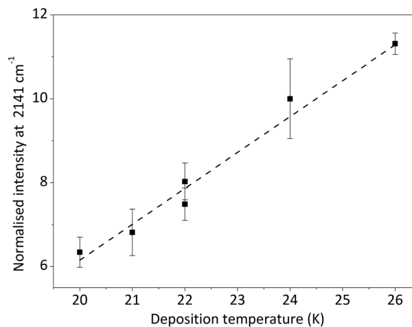
Fig. 4 Intensity measured at 2141 cm^{-1} in the RAIR spectra normalized by the total area of the \nu CO band for each spectrum, as a function of deposition temperature. The dotted line results from a linear fit of the data and is only presented here to guide the eye.
