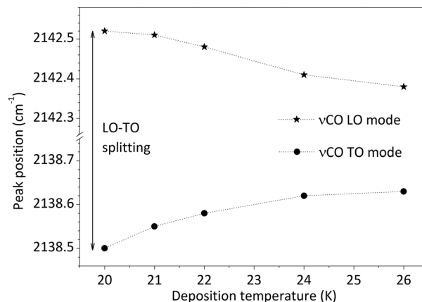
Fig. 3 Peak position of the \nu CO LO (stars) and TO (circles) modes of 5 ML CO films deposited on 300 nm silica, as a function of deposition temperature, deduced from fits to experimental data. The lines are a guide for the eye. Errors in frequencies are \pm 0.01 and \pm 0.02 cm^{-1} for LO and TO, respectively. Data are collated in Table 2, Section 3.1.
