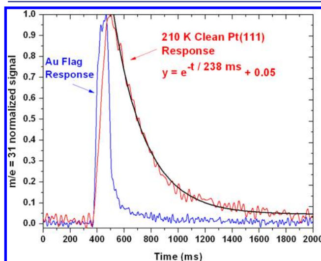
Figure 5. Normalized mass spectrometer signal versus time during the 2000 ms pulse cycle of methanol gas impinging on a Pt(111) surface held at 210 K, averaged over the first 30 pulses at the lowest coverage. The 100 ms pulse strikes the surface from \sim 380 to 480 ms on this scale. The slow desorption of methanol from the Pt(111) surface is apparent in the broad tail of the mass spectrometer response after this (red trace), which is fitted to an exponential decay with a 238 ms time constant (smooth black curve). For reference, the signal from the same 100 ms pulses of methanol after impinging on a room-temperature Au flag, where the molecules desorb rapidly, is also shown (blue trace).
