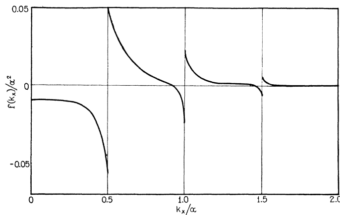
Fig. 6. Values of f(k_x)/\alpha^2 for the potential function V = (\hbar^2/8\pi^2\mu) [3 \cos (\alpha x)/4 - 3 \cos(2\alpha x)/10 + \cos(3\alpha x)/20]
