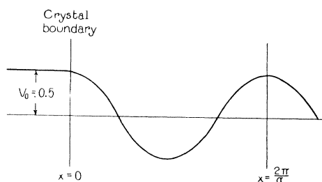
Fig. 7. Assumed form of potential energy function.
