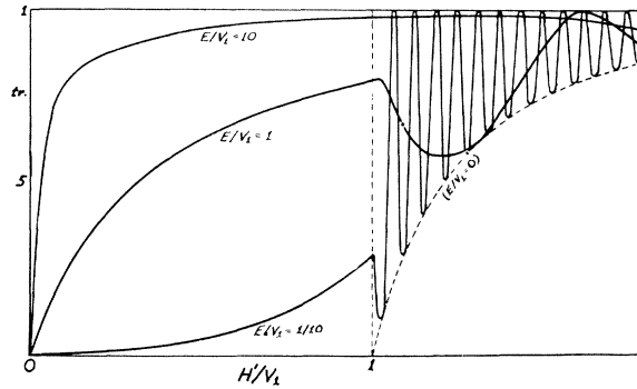
Fig. 2. Probability of transmission at a potential wall of height V_1 . ( E is the energy of a particle of de Broglie wave-length equal to the thickness of the wall.)
