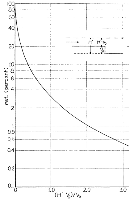
Fig. 1. Probability of reflection at a sudden drop in the potential energy.
