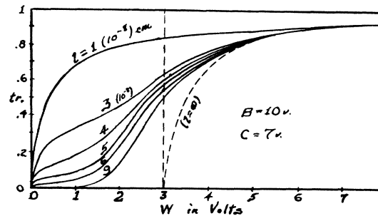
Fig. 4. Transmission probabilities for the potential barrier of Fig. 3.
