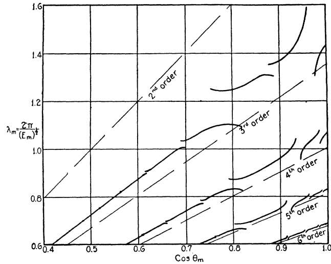
Fig. 9. Values of electronic wave number and angle of incidence of electron beam for strong regularly reflected beam. The crystal is nickel, the surface the 111 plane. Broken lines indicate positions of analogous x-ray reflection.
