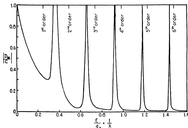
Fig. 8. Relative intensity of the regularly reflected beam as a function of the electronic wave number. The incident beam is normal to the 111 surface of a nickel crystal. Lines marked 1st order, etc., indicate positions of strong x-ray reflection for the same crystal.
