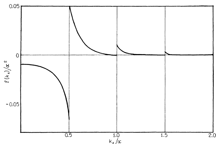
Fig. 5. Values of f(k_x)/\alpha^2 for the potential function V = (\hbar^2/8\pi^2\mu)(\cos \alpha x/2)
