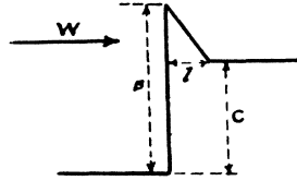
Fig. 3. Form of the potential energy function used by Georgeson.
