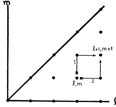
FIG. 4. The solution Y_{l+1}^{m+1} can be reached from Y_l^m by moving along either path with the appropriate operators.
