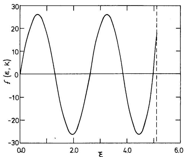
Fig. 1. Equation (15) plotted for the case of an electron in a finite rectangular potential well of depth 100 eV and width 2 \text{ \AA} . The zeros of the curve correspond to the permissible energy eigenvalues. The dashed line indicates the top of the well.
