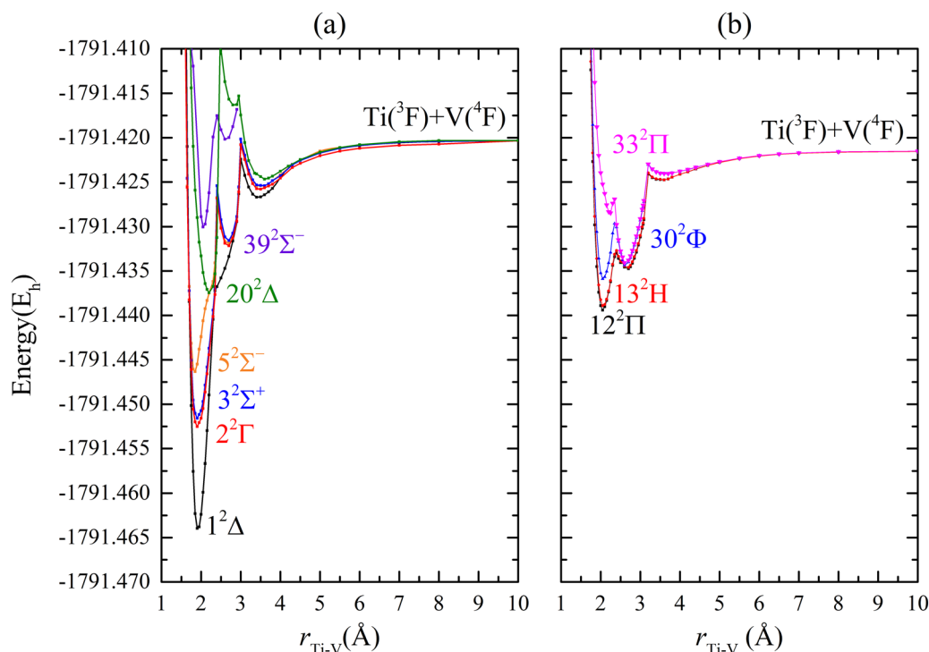
Fig. 3 Potential energy curves of the ten lowest doublet states of TiV at the MRCI/cc-pVQZ level of theory: (a) 1^2\Delta , 2^2\Gamma , 3^2\Sigma^+ , 5^2\Sigma^- , 20^2\Delta , 39^2\Sigma^- and (b) 12^2\Pi , 13^2H , 30^2\Phi , 33^2\Pi .
