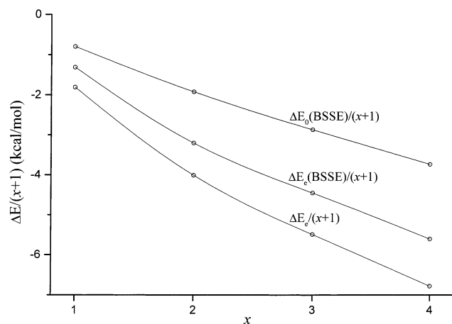
Figure 6. Variation of the “average” dissociation energies, \Delta E_e/(x+1) , \Delta E_c(\text{BSSE})/(x+1) , and \Delta E_0(\text{BSSE})/(x+1) of the global minima (m1) with cluster size x at the MP2/avdz level.
