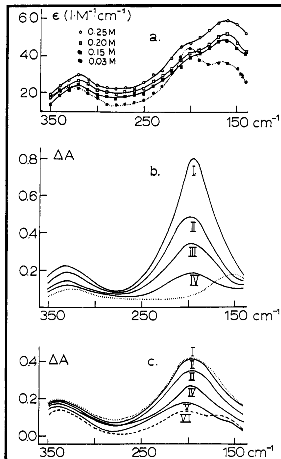
Figure 1. Infrared spectra (140–350 \text{cm}^{-1} ) (Beckman IR11 spectrometer): (a) \text{NaAlBu}_4 in \text{C}_6\text{H}_{12} ; (b) —, \text{NaAlBu}_4 in THF (I, 0.5 M ; II, 0.3 M ; III, 0.2 M ; IV, 0.1 M ); ····, \text{KAlBu}_4 in THF (0.35-mm path length); (c) 0.02 M \text{NaAlBu}_4 in \text{C}_6\text{H}_{12} (4-mm path length). R = mole ratio THF: \text{Na}^+ (I, R = 5.0; II, R = 4.0; III, R = 2.0; IV, R = 1.2; V, R = 0.8; VI, R = 0.3). Solvent and cell absorption have been subtracted.
