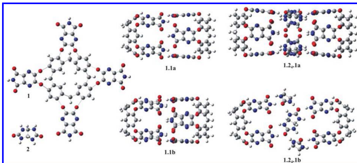
Figure 2. Structures of the cavitand 1 and glycoluril 2 components and structures of the cages 1.1 and 1.2.4.1 . H atoms = white spheres, C = gray spheres, O = red spheres, and N = blue spheres.
