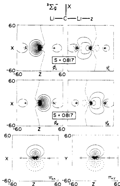
Figure 8. The GVB valence orbitals of the {}^3\Sigma_g^- state of \text{Li}_2\text{C} at a C-Li bond length of 3.70 bohrs.
