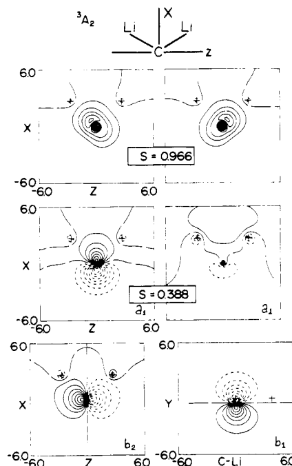
Figure 10. The GVB valence orbitals of the {}^3A_2 state of \text{Li}_2\text{C} at a bond length of 3.80 bohrs and bond angle of 90^\circ .
