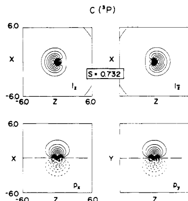
Figure 2. The GVB valence orbitals l r , l l , p x , and p y for the 3 P state of C. The plots have uniformly spaced contours with increments of 0.05 au. Positive contours are indicated by solid lines, negative contours are indicated by dotted lines, and nodal planes are indicated by long dashes. The same conventions are used for all plots.
