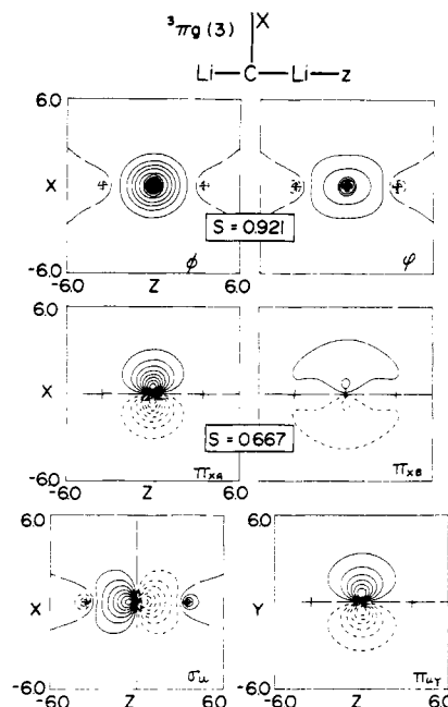
Figure 9. The GVB valence orbitals of the {}^3\Pi_g(3) state of \text{Li}_2\text{C} at a C-Li bond length of 3.50 bohrs.
