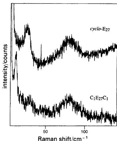
Fig. 9 Low-frequency Raman spectra ( 5\text{--}140\text{ cm}^{-1} ) of crystalline cyclo-E 27 and linear C 1 E 27 C 1 (as indicated). For clarity of presentation the intensity scales of the two spectra are displaced relative to one another.
