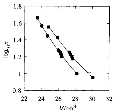
Fig. 1 Calibration curves for GPC System B. Logarithm of chain length in E units, i.e. n for (●) cyclic oligomers and n + 1 for (■) linear oligomers, vs. elution volume ( V ). (□) Denotes a sample of cyclo - E_{10} prepared in Prof. Gibson's laboratory.
