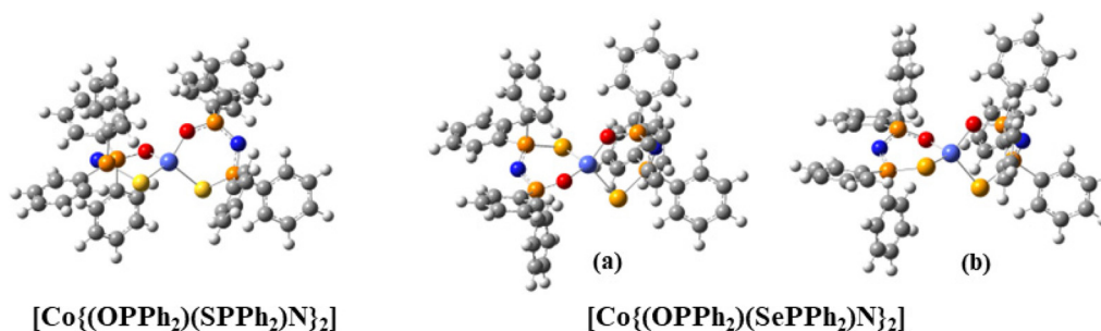
Fig. 7 The lowest in energy isomers of the \text{CoO}_2\text{E}_2 , E = S, Se complexes. Color coding: Co (light blue), O (red), S (yellow), Se (light brown), N (blue), C (gray).
