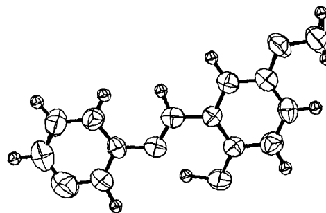
Fig. 3. Vibrational ellipsoids [50% probability level (Johnson, 1965)] of (II) projected on the mean plane of the molecule.
