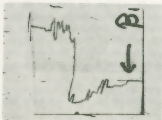
Fig. 3. \text{Br}_2 Addition an Furan
