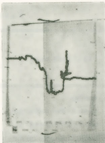
Fig. 4. \text{Br}_2 - Addition an Tetralin.
