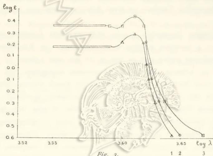
Fig. 3. 2 = AgJ-Grundkörper 0 = \frac{I}{20} NaClO 4 und \frac{I}{20} TiClO 4 1 = \frac{n}{20} - KJ 3 = \frac{n}{20} - AgClO 4
