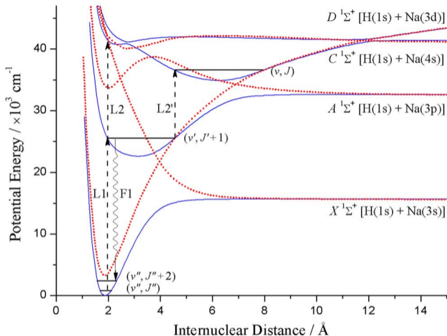
FIG. 1. The 4 lowest 1\Sigma^+ states of the NaH and the experimental scheme used to investigate the C \ 1\Sigma^+ state (blue solid lines: adiabatic potential curves; red dotted lines: diabatic potential curves).
